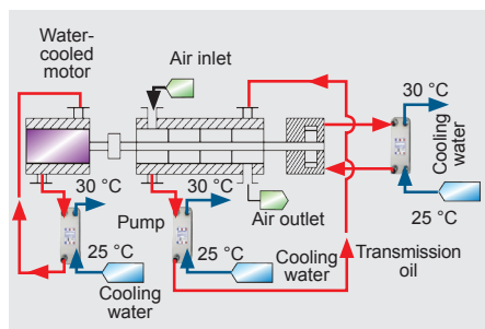
Vacuum pump
