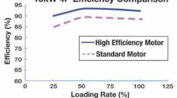
15kW 4P Efficiency Comparison
