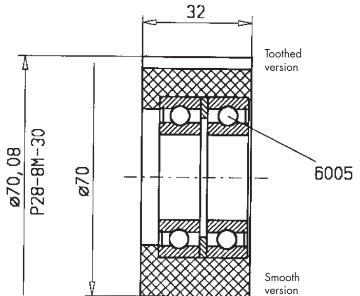
Plastic idlers with bearings
